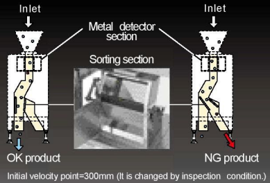
Schematics of sorting operation
